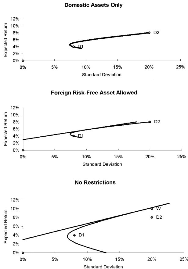
Fig. 1. Gains from international risk sharing: restricted versus unrestricted efficient portfolio frontiers
