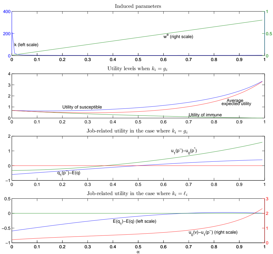
Figure 1: Utility and output levels in “high- w^e ” stochastic model
