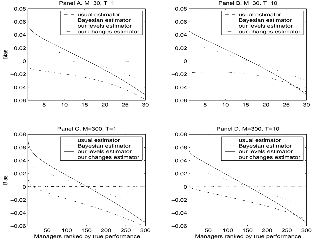
Figure 1. Bias of alternative performance estimators with respect to the traditional performance measure.
